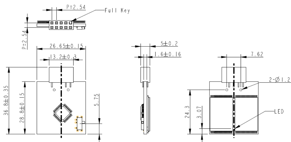
Figure 7-4 Type D Dimensions
