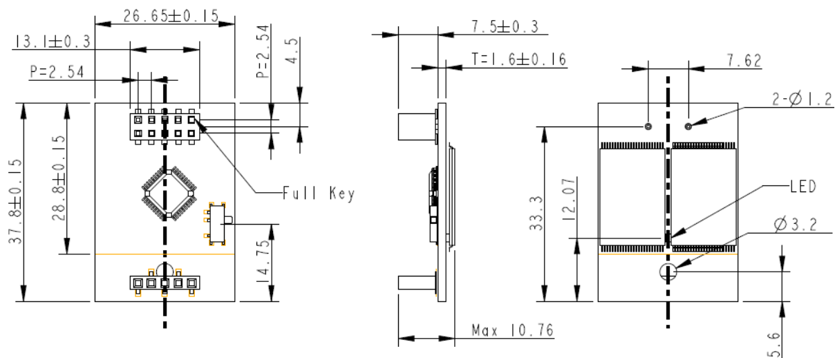
Figure 7-2 Type B Dimensions
