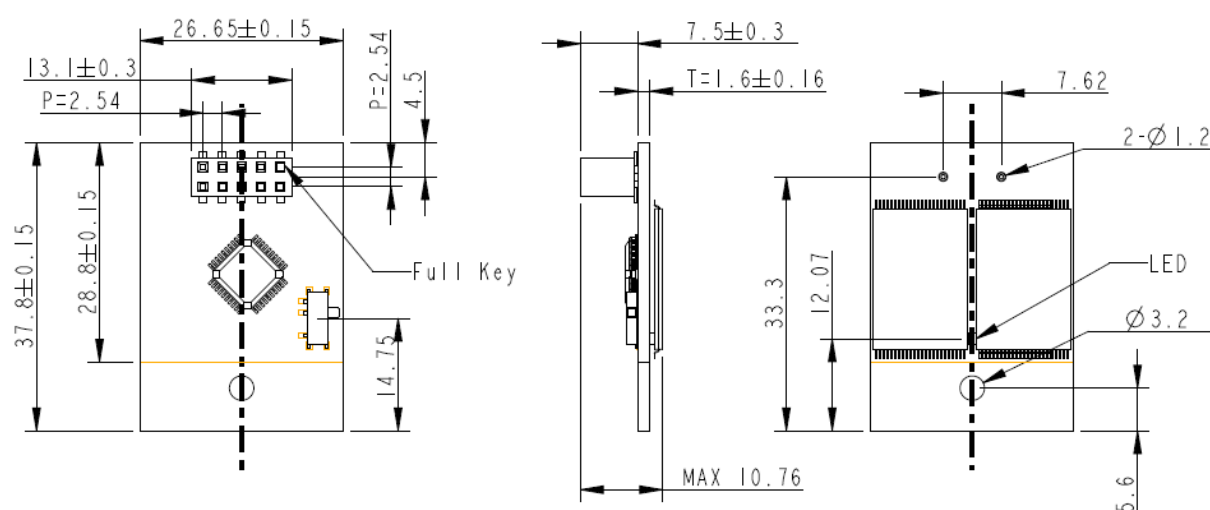
Figure 7-3 Type C Dimensions
