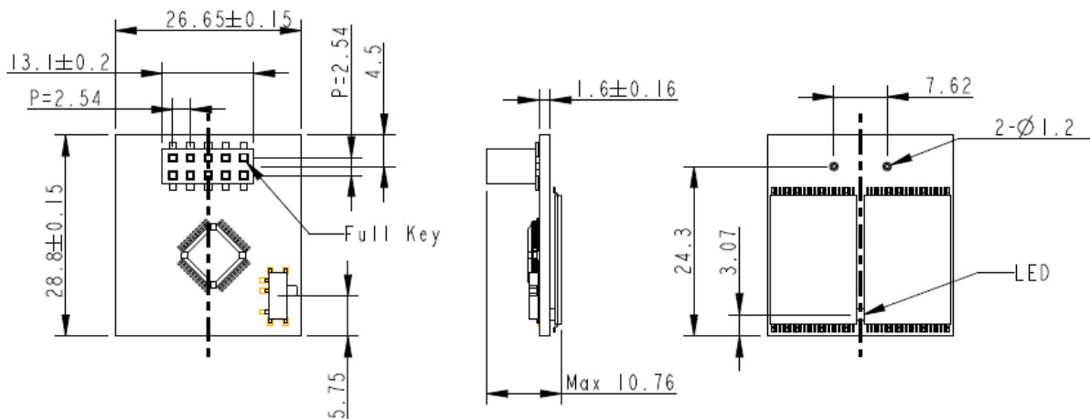
Figure 7-1 Type A Dimensions
