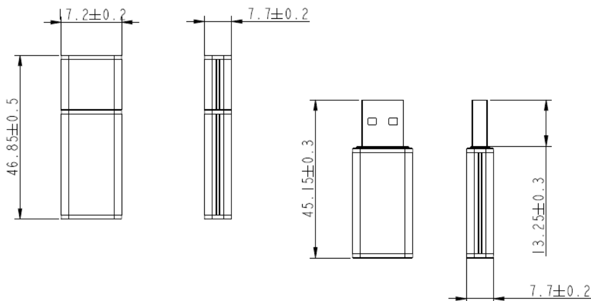
Figure 6-1 Physical Dimensions
