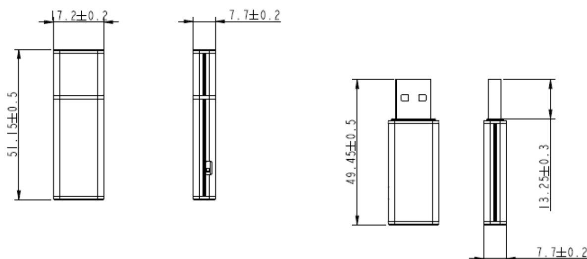
Figure 6-1 Physical Dimensions
