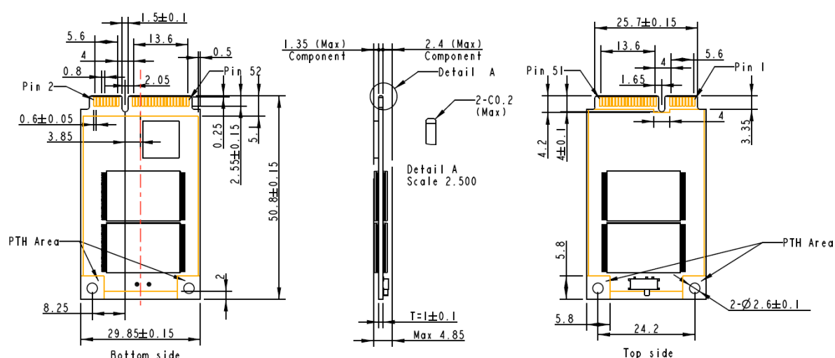
Figure 9-1 Physical Dimensions
