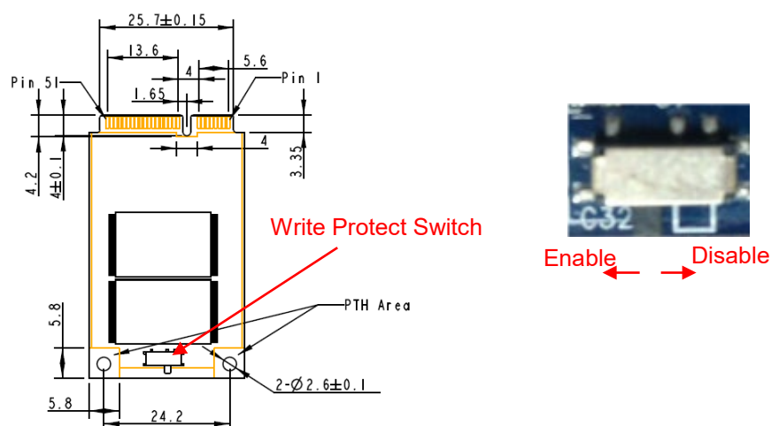
Figure 9-2 Write Protect Switch
