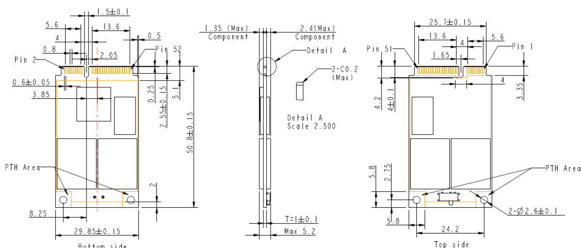
Figure 9-1 Physical Dimensions
