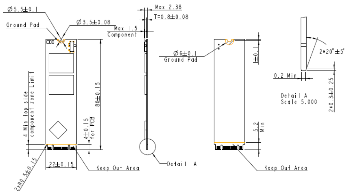
Figure 9-1 Single-sided Dimensions
