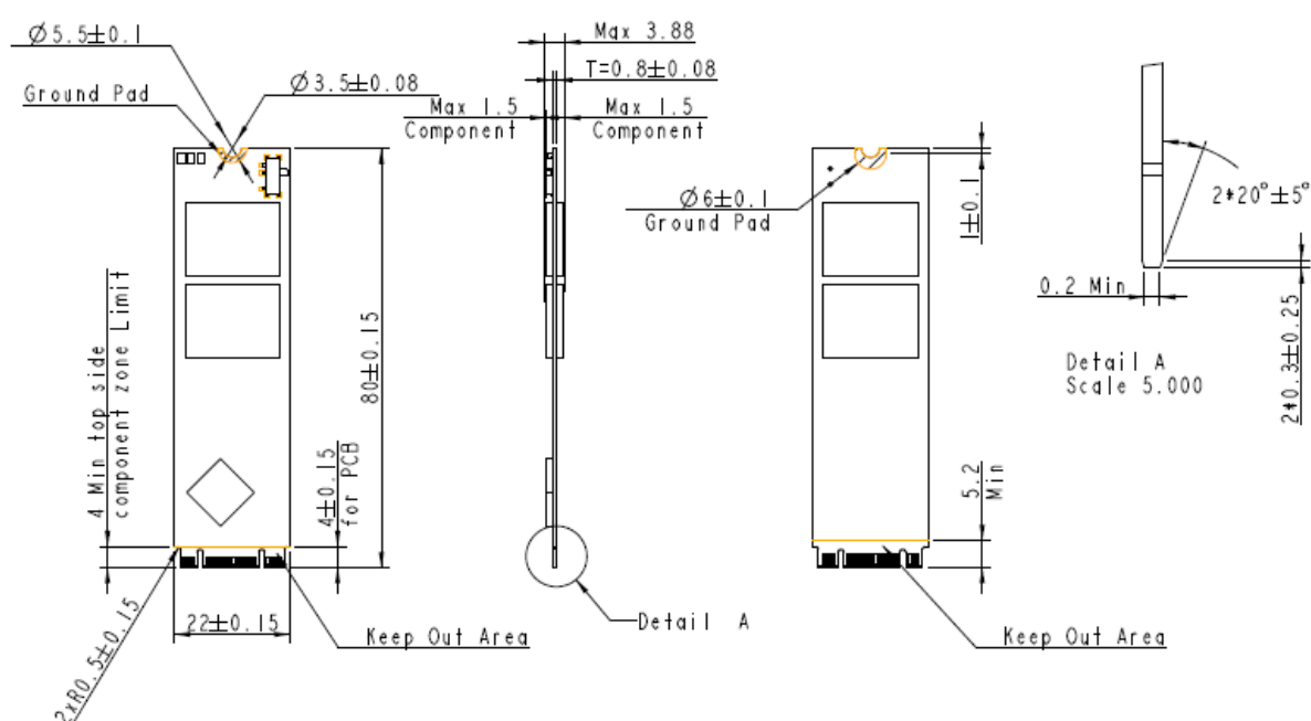
Figure 9-2 Double-sided Dimensions
