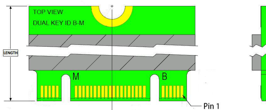
Figure 3-1 Pin Connectors
