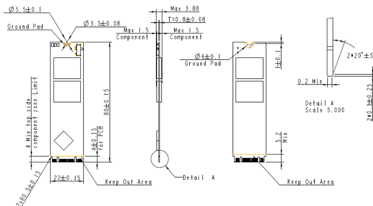
Figure 9-2 Double-sided Dimensions
