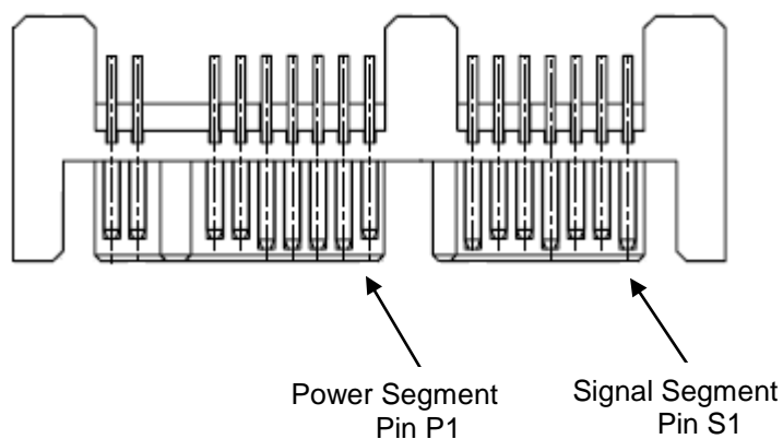
Figure 1-1 Micro-SATA Connectors
