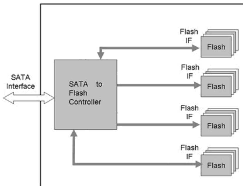
Figure 1-1 Apacer SAFD25M4-M block diagram
