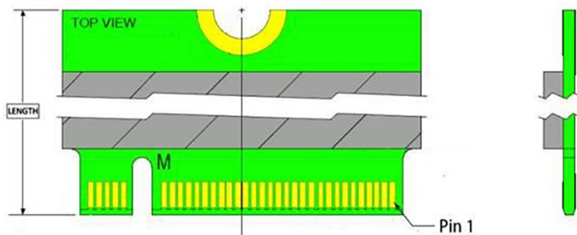
Figure 3-1 Pin Connectors
