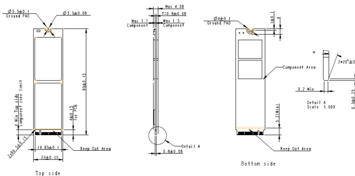
Figure 10-2 Double-sided Dimensions
