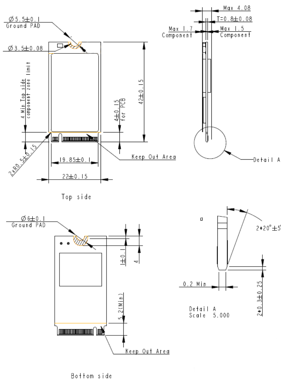
Figure 10-1 Physical Dimensions
