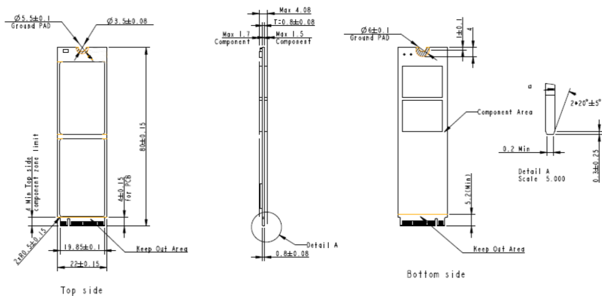
Figure 10-2 Double-sided Dimensions
