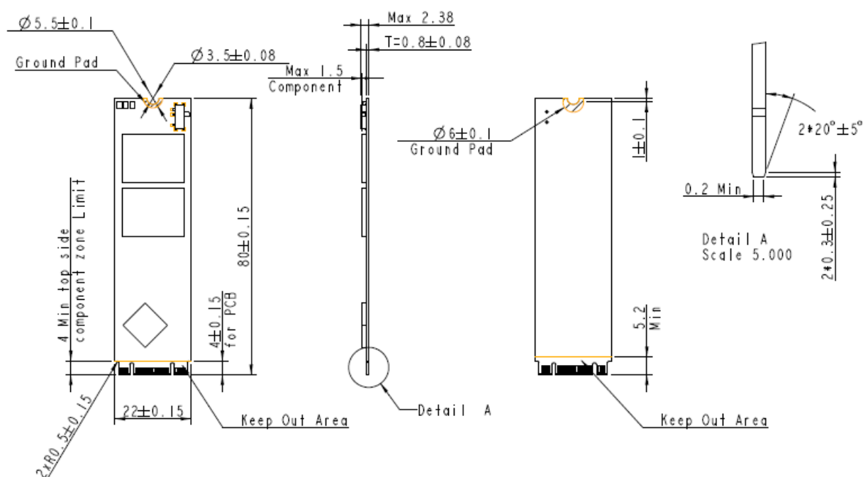
Figure 9-1 Single-sided Dimensions
