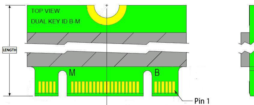
Figure 3-1 SATA Connectors
