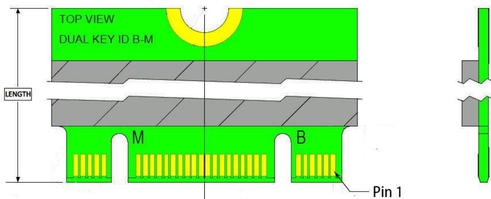
Figure 3-1 SATA Connectors
