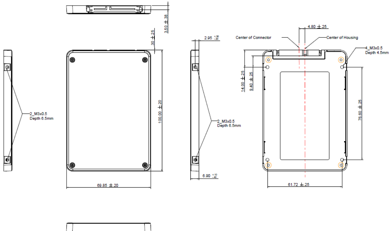
Figure 6-1 7mm Housing Physical Dimensions
