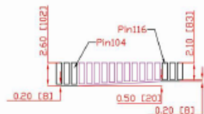
Detail D
