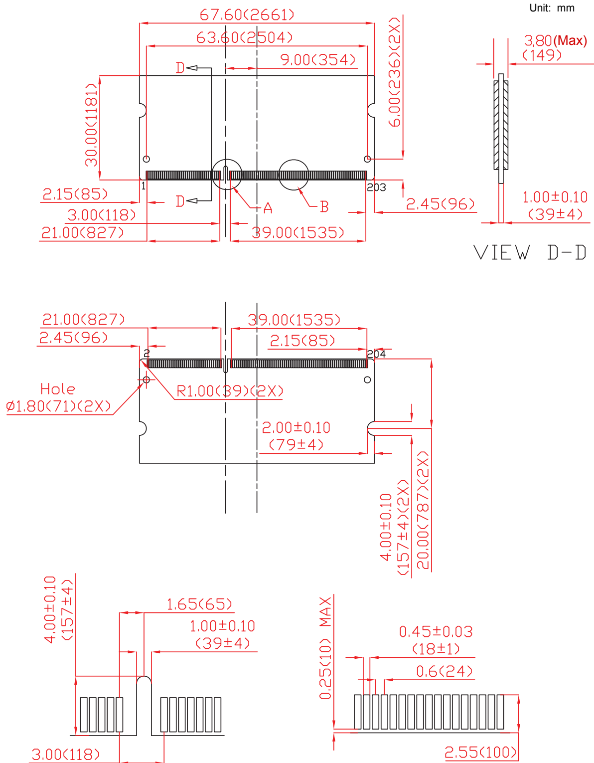
Detail A 30μ inch gold finger
