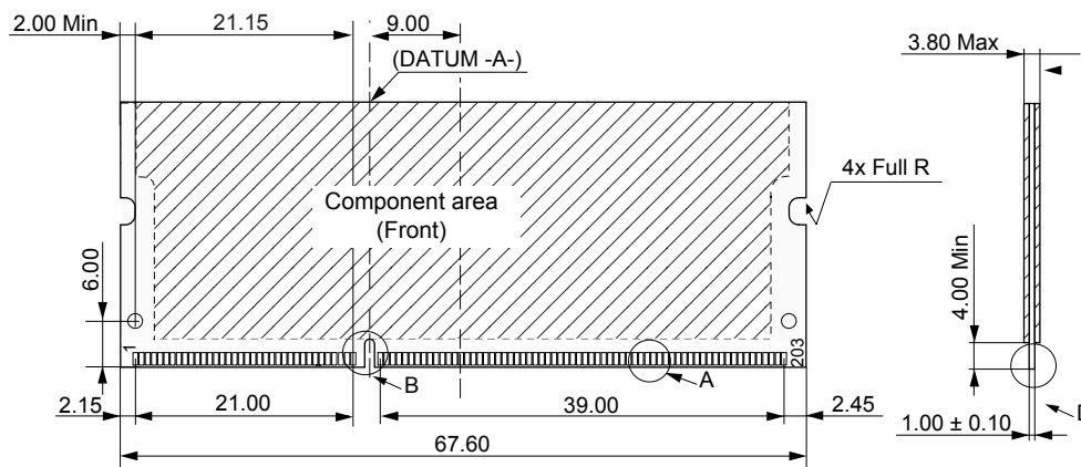
Back side
