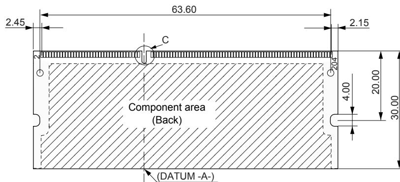
Detail A
