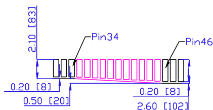
Detail C
