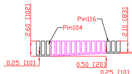
Detail D
