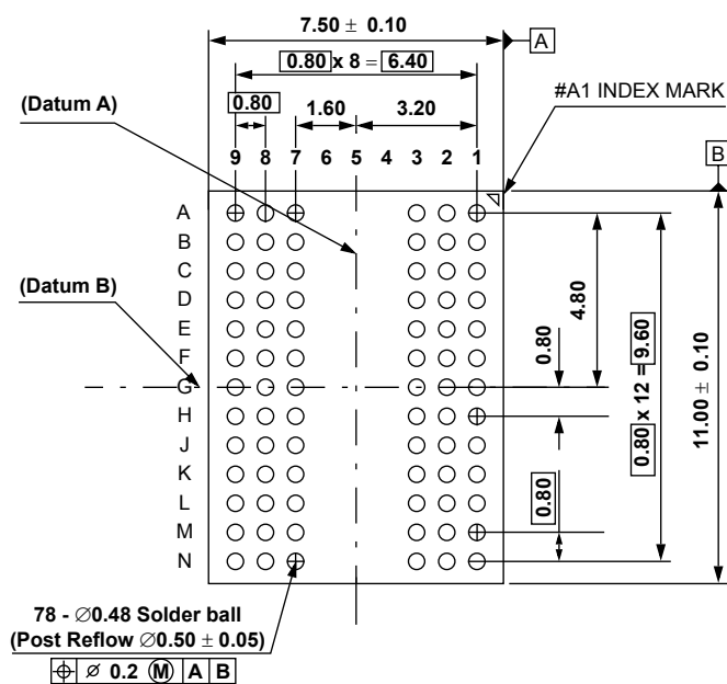
BOTTOM VIEW
