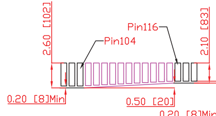
Detail D
