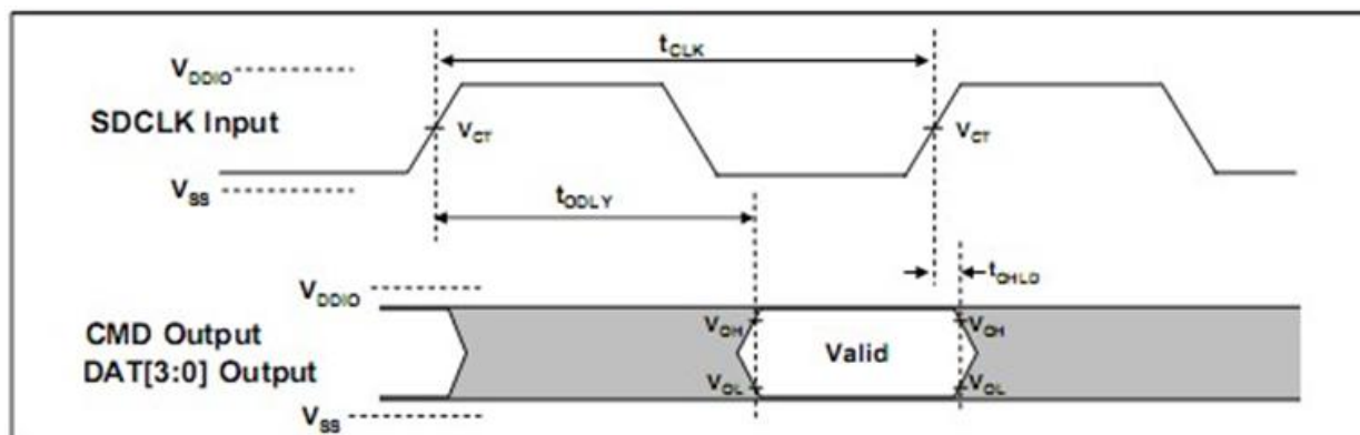
Output Timing of Fixed Date Window u
