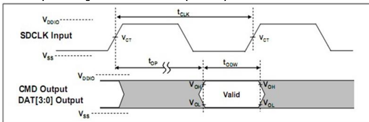
Output Timing of Variable Data Window u
